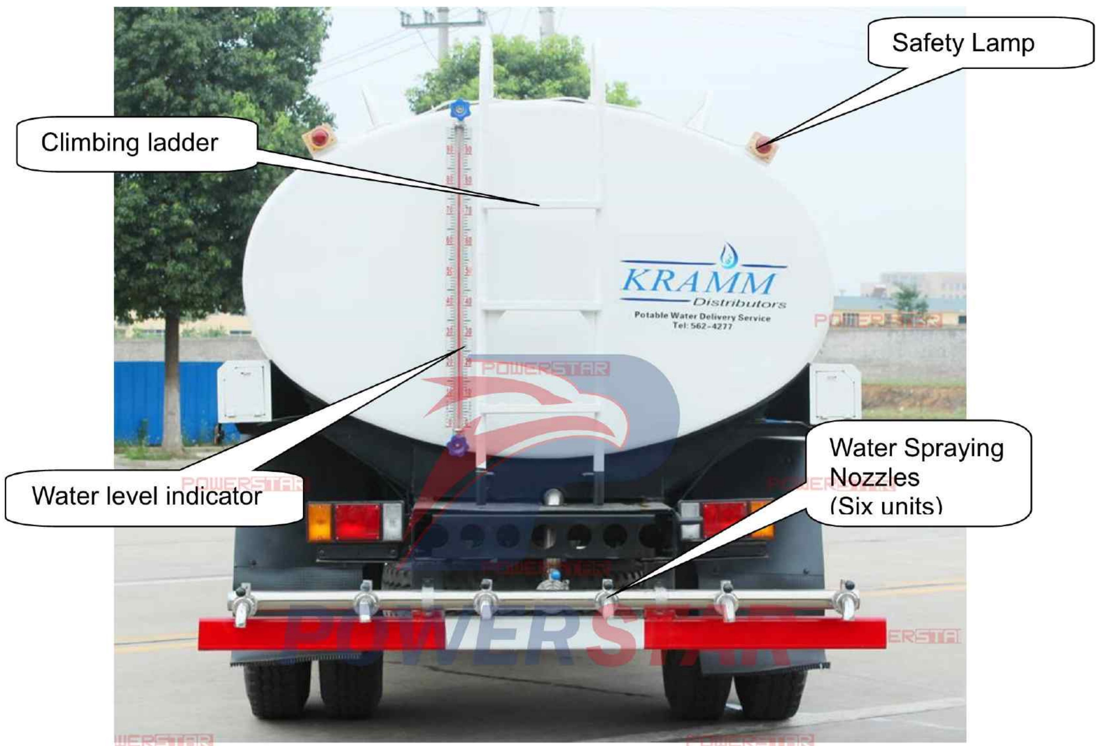
Rear of the Tank: Climbing ladder, water discharging nozzles, safety lamp and water level indicator.
