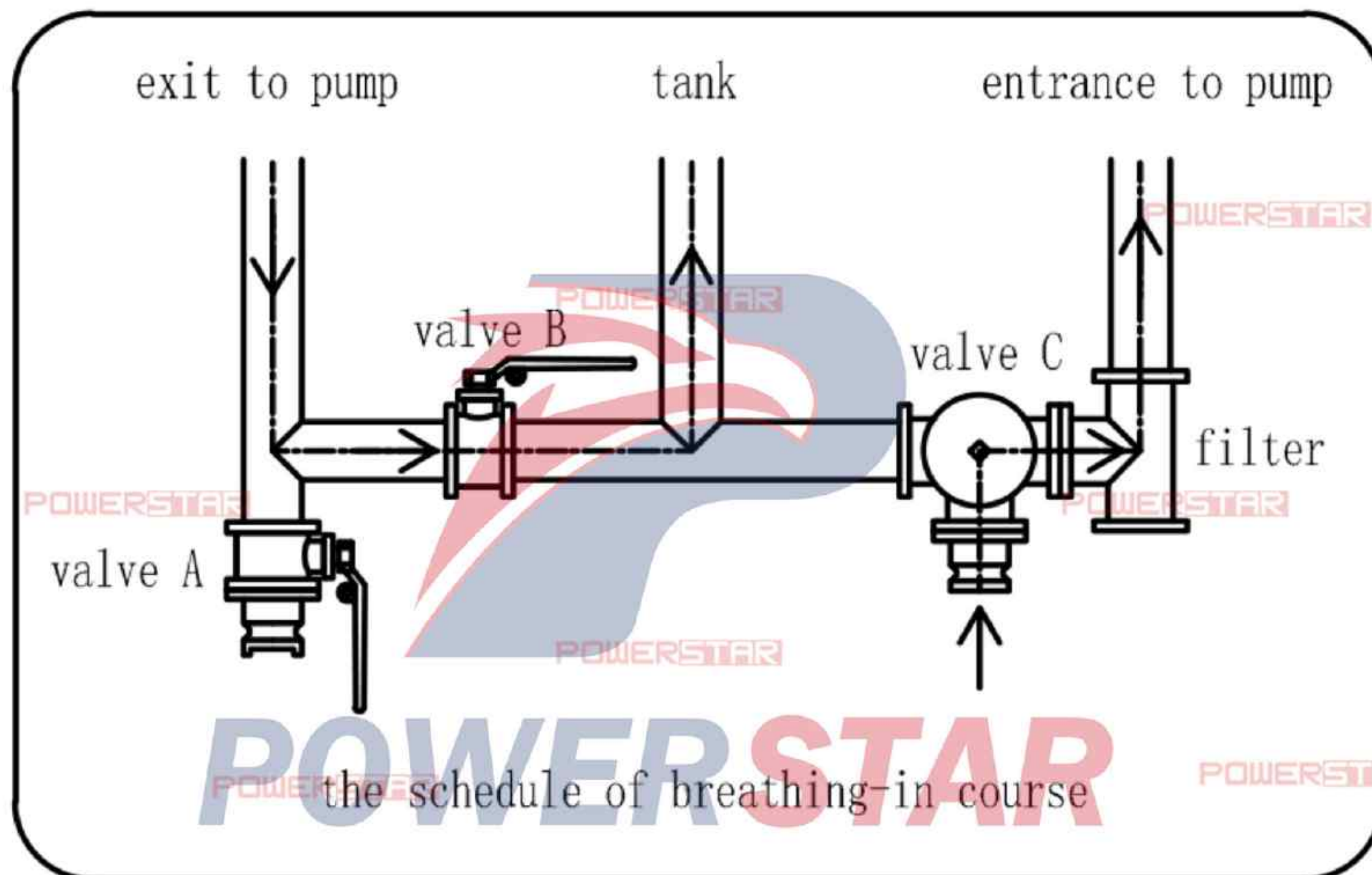
(Pump-In Process Working principle)
