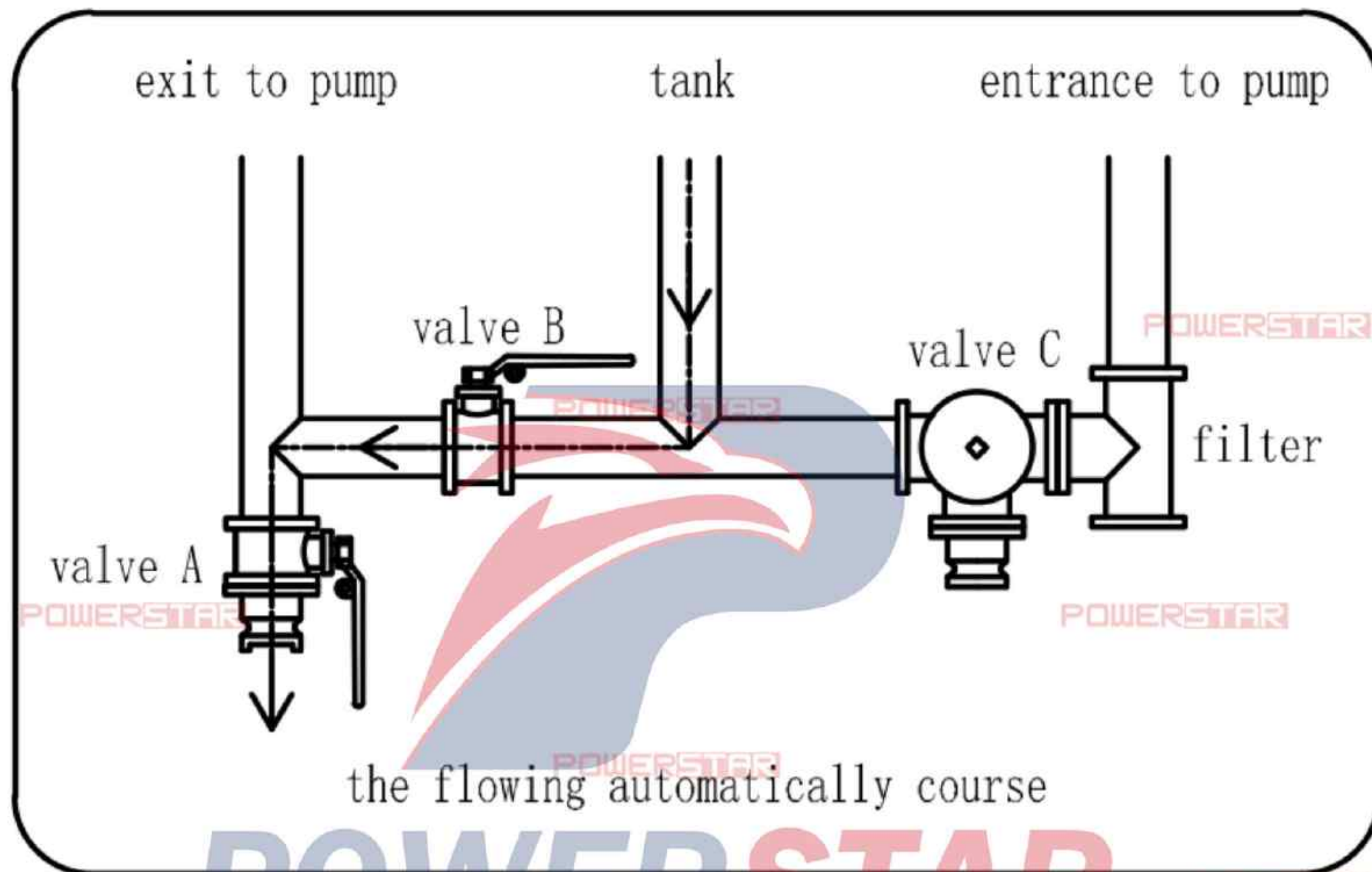
(Flowing Automatically Process Working principle)
