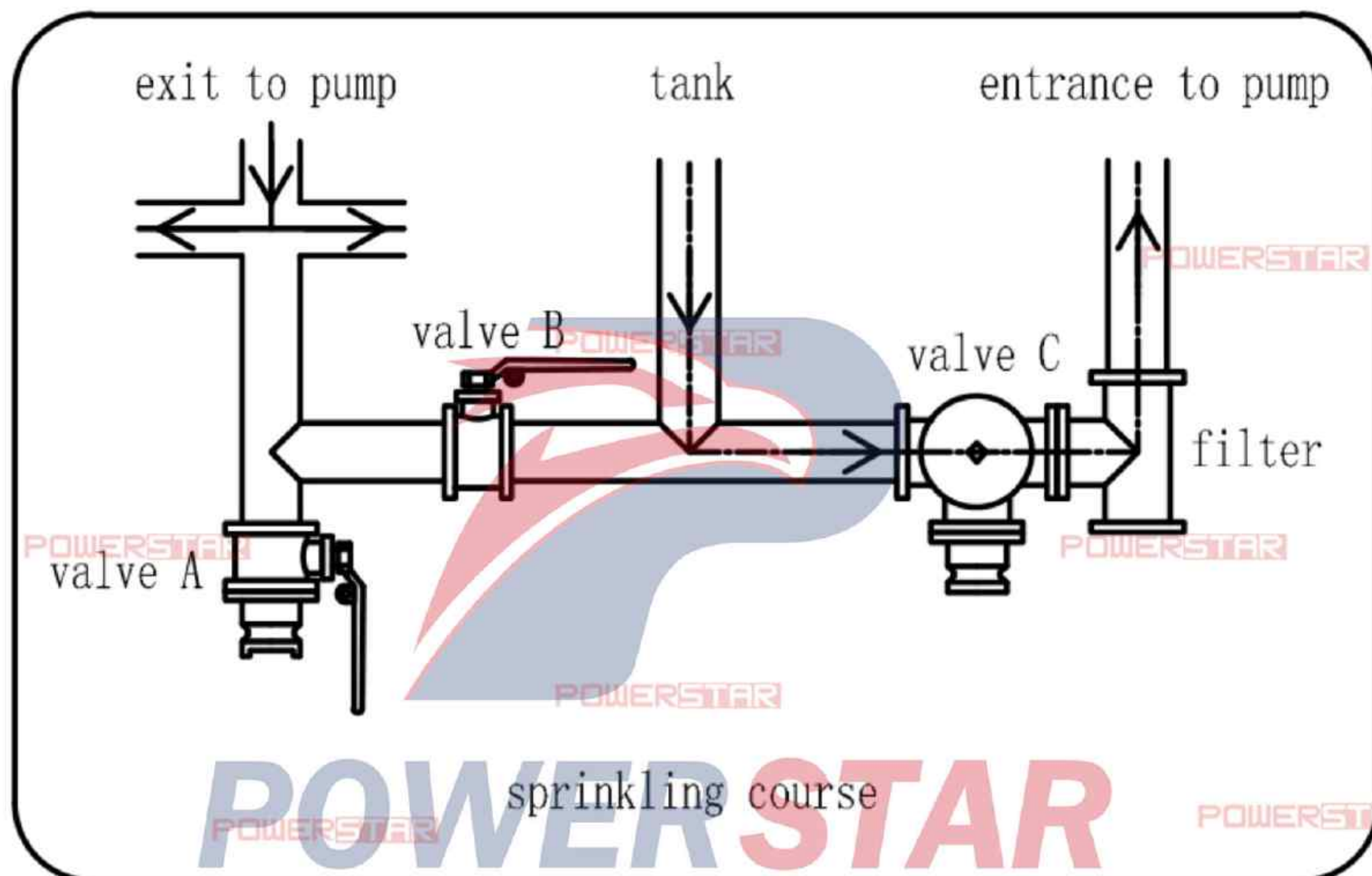
(Pump-Out Process Working principle)
